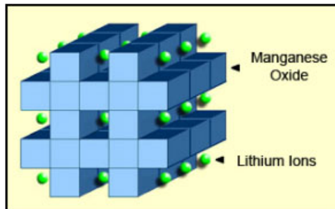
Figure 4: Li-manganese structure.
